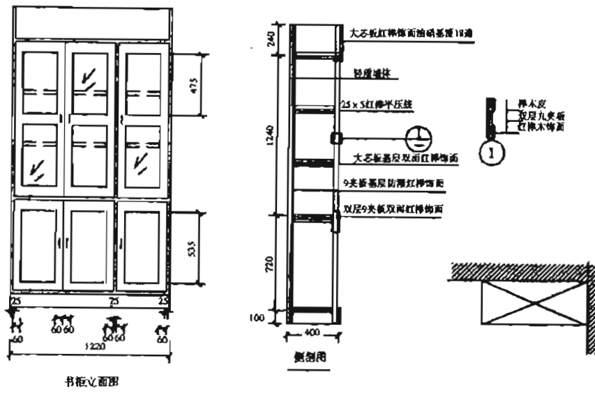
18-112 附墙书柜
