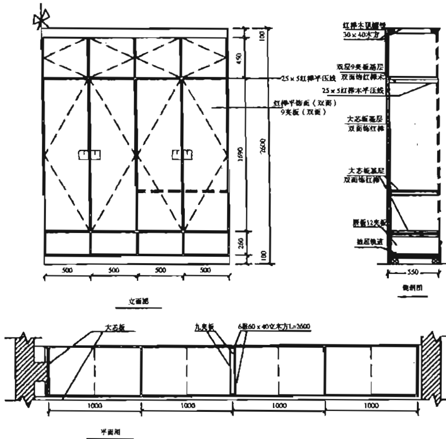
18-111 隔断木衣柜
