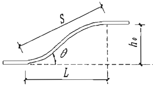
弯起钢筋图
