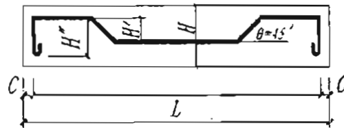
弯起钢筋两端带直钩图
