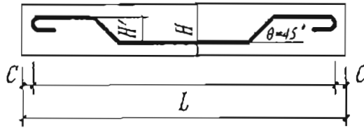
弯起钢筋图
