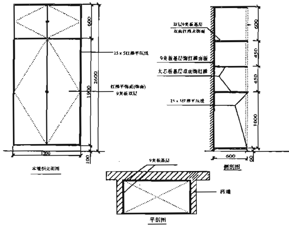
18-109 嵌入式木壁柜
