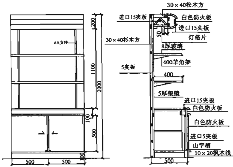
18-98 货架2
